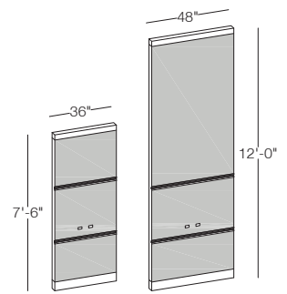
Off-Module Beltline Electric
