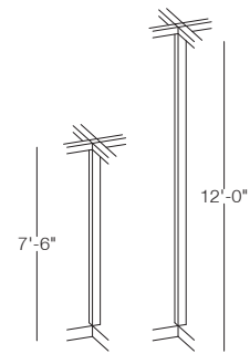
4-Way Furniture Post
