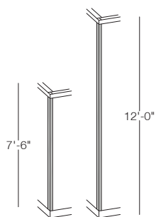
2-Way Building 'L' Condition
