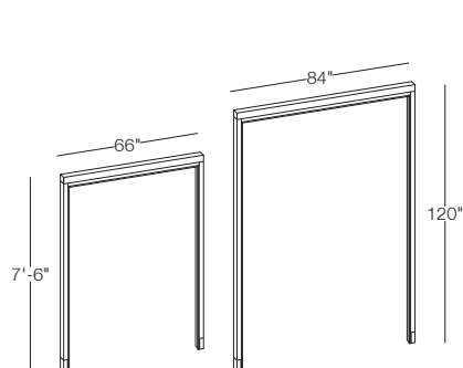
Full Height Double Door Frame
