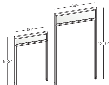
Glass Transom Double Door Frame
